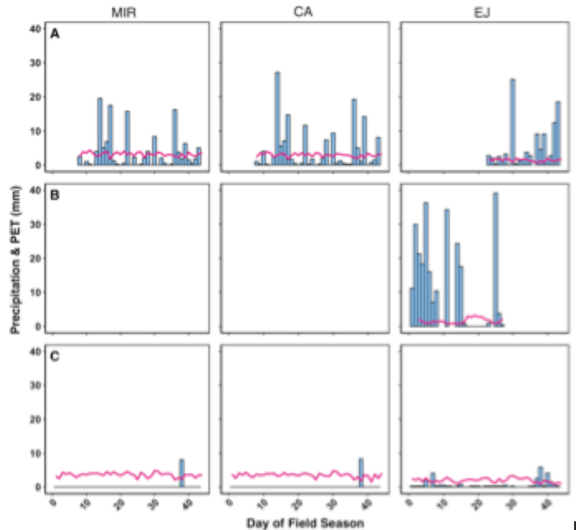
Figure 1. Daily total precipitation (blue bars) and potential evapotranspiration (PET, pink lines) for all three field sites (located at 320, 520, and 670 m, respectively). Panels A, B and C represent field seasons one, two and three, respectively. This graphic visually represents plant water supply (blue bars) versus plant water demand (pink lines). Note that meteorological data is missing from MIR/CA for FS2 so no graphics could be rendered.
